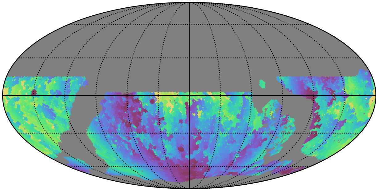
noroll_mjdp180_v3.4_10yrs WFD g band: Min solarElong
