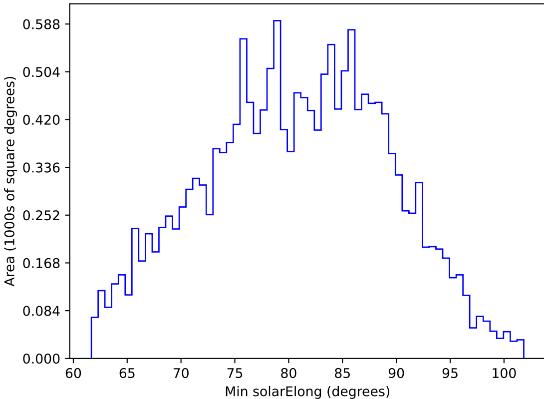
noroll_mjdp180_v3.4_10yrs WFD g band: Min solarElong
