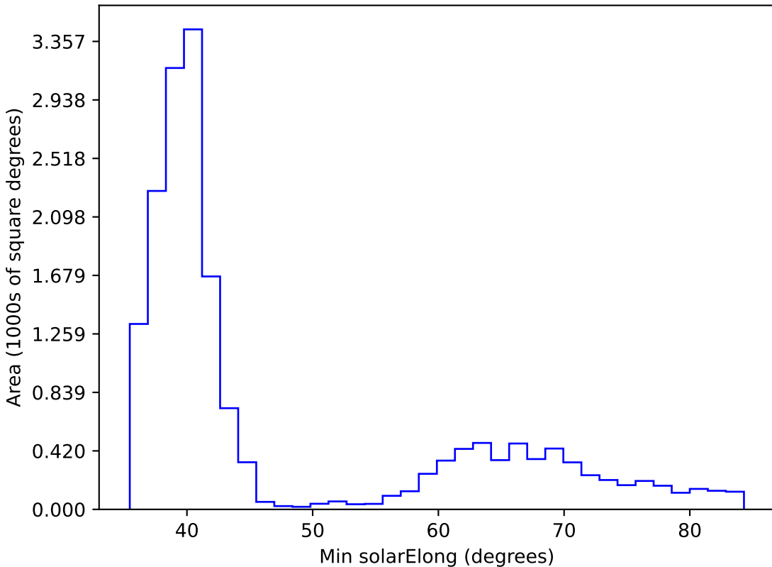
noroll_mjdp180_v3.4_10yrs WFD all bands: Min solarElong
