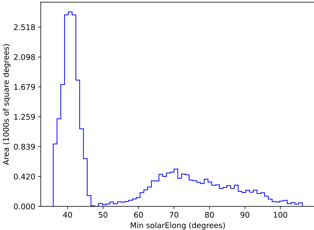
noroll_mjdp180_v3.4_10yrs All sky z band: Min solarElong
