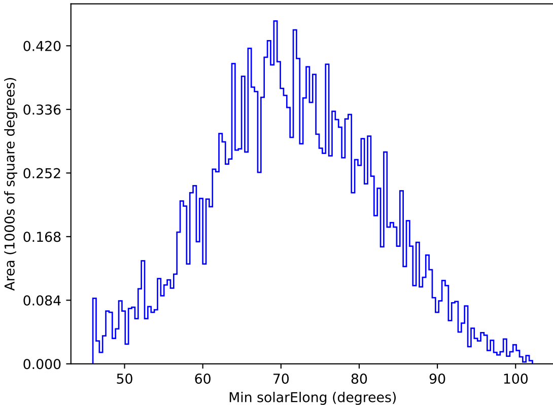
noroll_mjdp180_v3.4_10yrs All sky y band: Min solarElong
