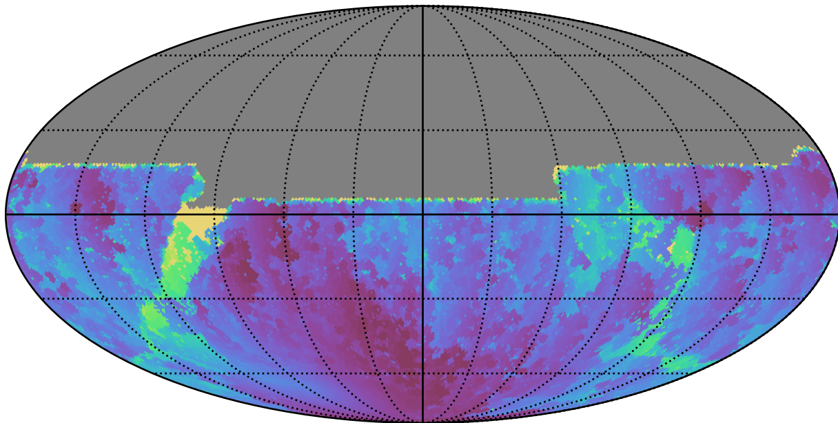
noroll_mjdp180_v3.4_10yrs All sky u band: Min solarElong
