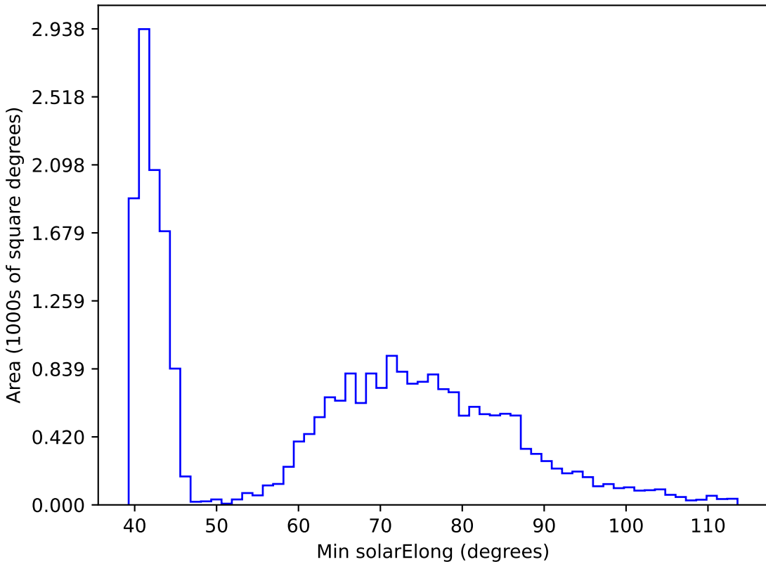
noroll_mjdp180_v3.4_10yrs All sky r band: Min solarElong
