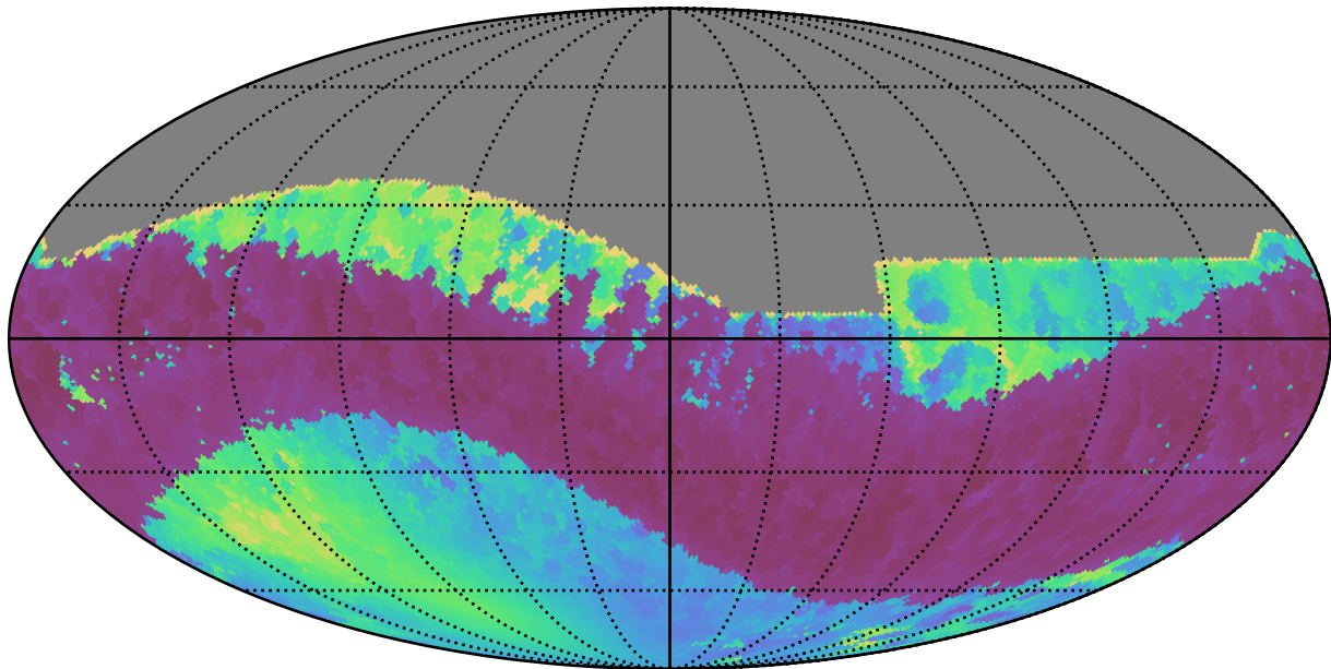
noroll_mjdp180_v3.4_10yrs All sky i band: Min solarElong
