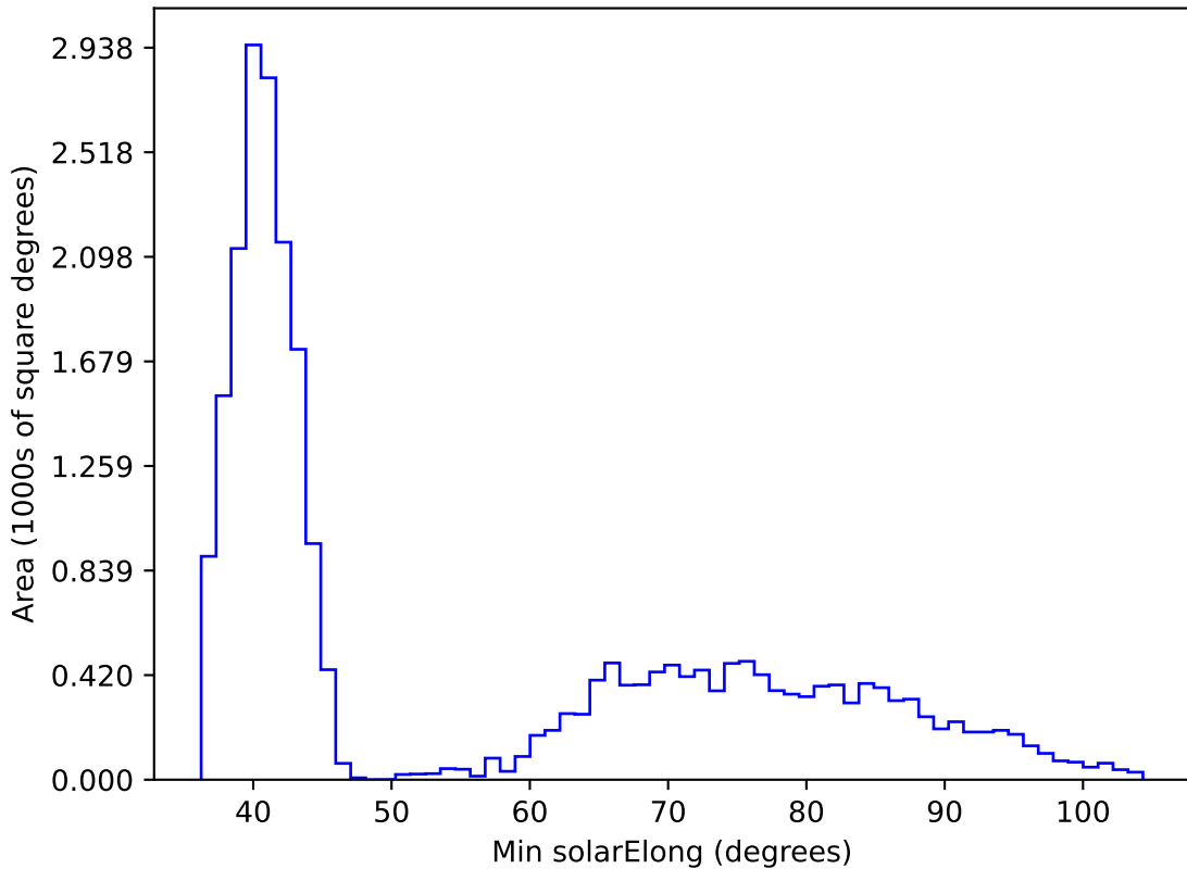
noroll_mjdp180_v3.4_10yrs All sky i band: Min solarElong
