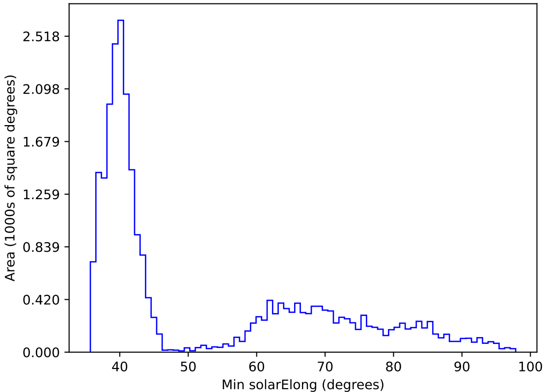
noroll_mjdp180_v3.4_10yrs All sky all bands: Min solarElong
