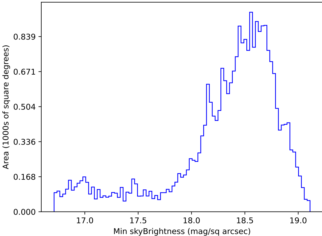
noroll_mjdp180_v3.4_10yrs Yr 1 z band: Min skyBrightness
