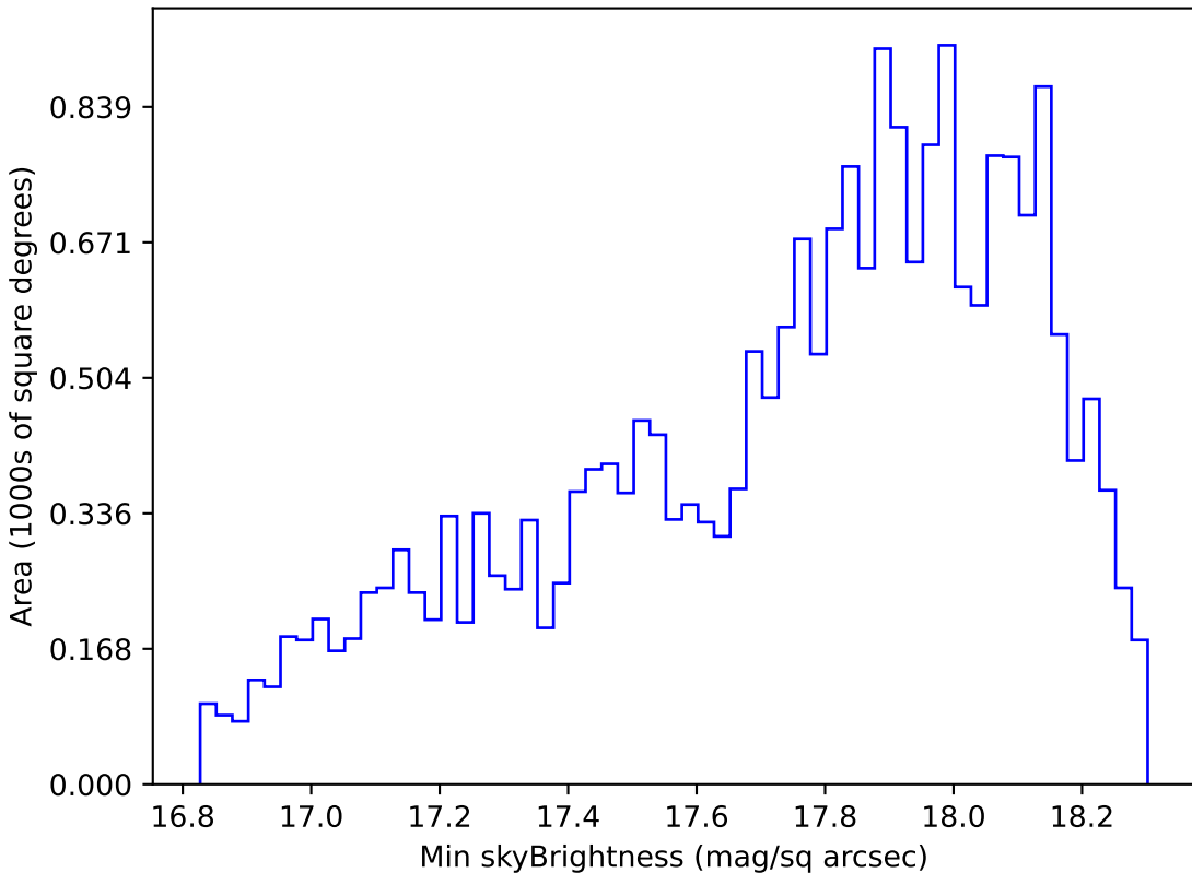
noroll_mjdp180_v3.4_10yrs Yr 1 y band: Min skyBrightness
