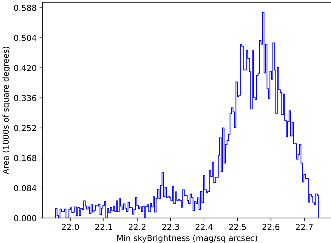
noroll_mjdp180_v3.4_10yrs Yr 1 u band: Min skyBrightness
