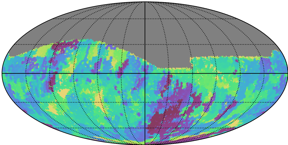
noroll_mjdp180_v3.4_10yrs Yr 1 r band: Min skyBrightness
