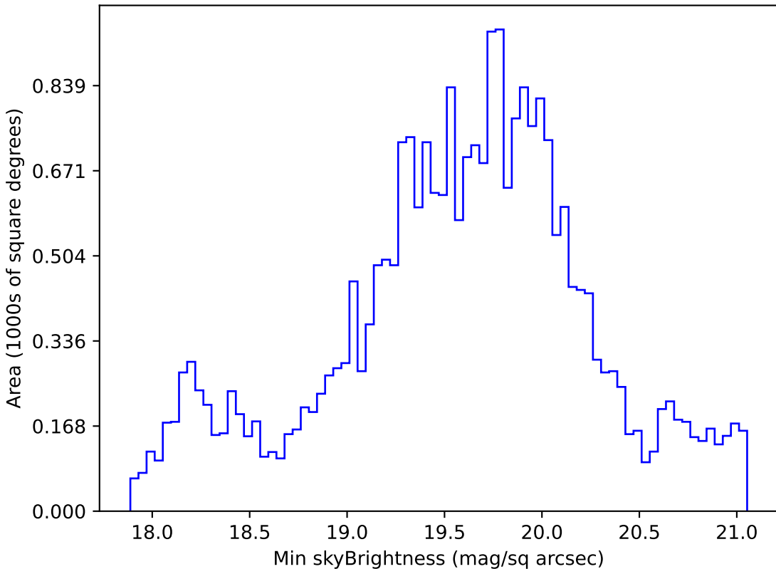
noroll_mjdp180_v3.4_10yrs Yr 1 r band: Min skyBrightness
