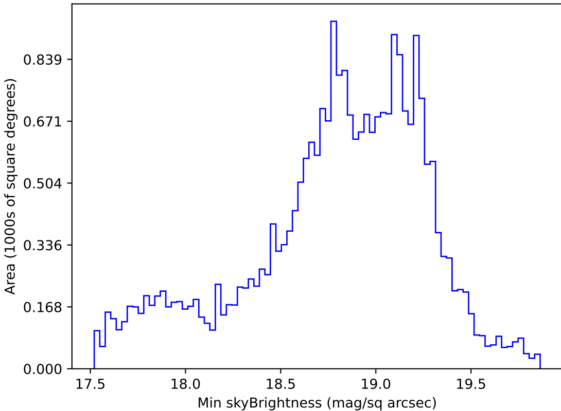
noroll_mjdp180_v3.4_10yrs Yr 1 i band: Min skyBrightness
