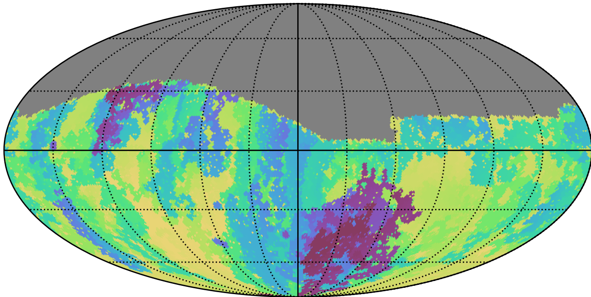
noroll_mjdp180_v3.4_10yrs Yr 1 g band: Min skyBrightness
