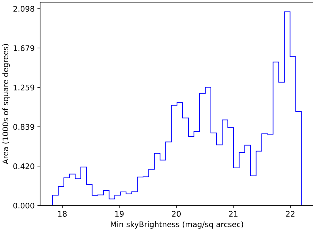
noroll_mjdp180_v3.4_10yrs Yr 1 g band: Min skyBrightness
