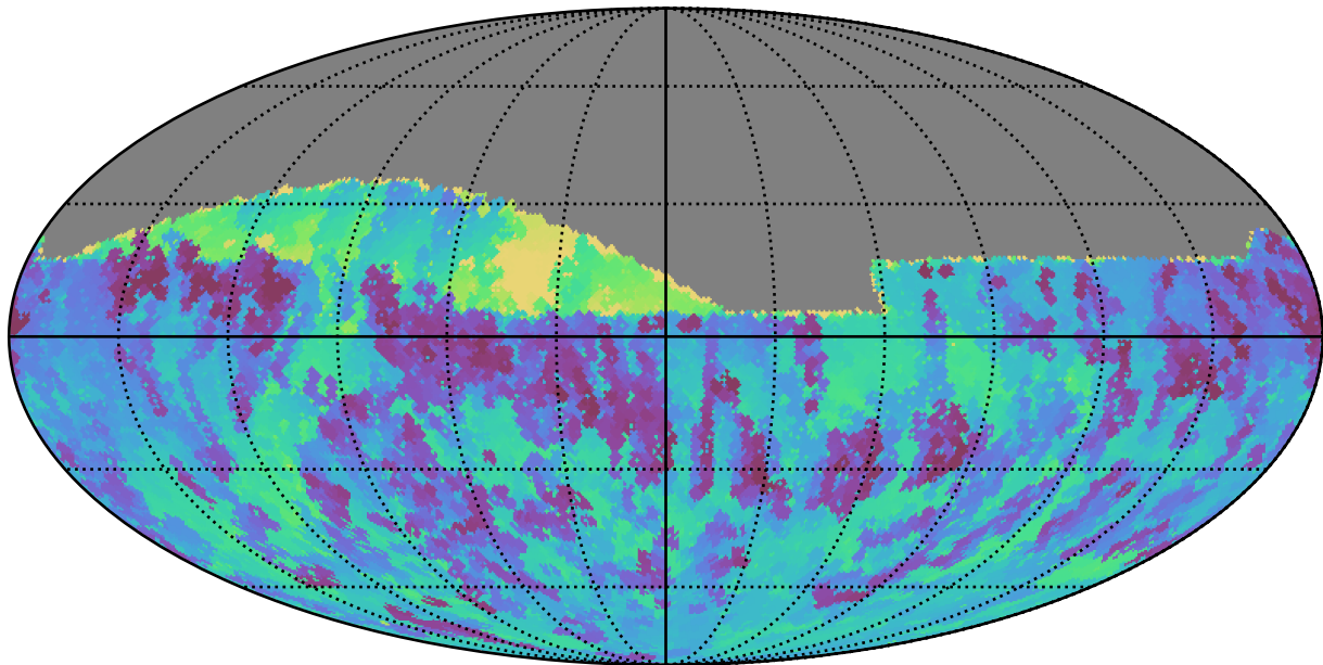
noroll_mjdp180_v3.4_10yrs Yr 1 all bands: Min skyBrightness
