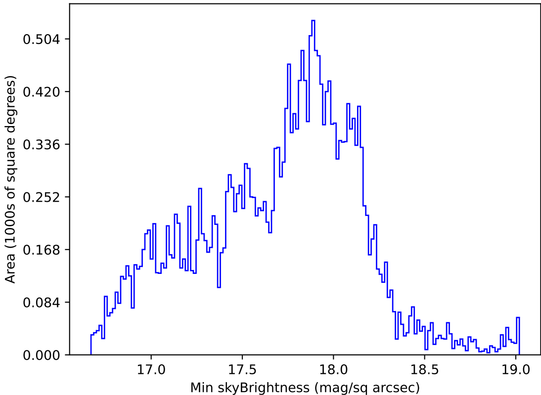
noroll_mjdp180_v3.4_10yrs Yr 1 all bands: Min skyBrightness
