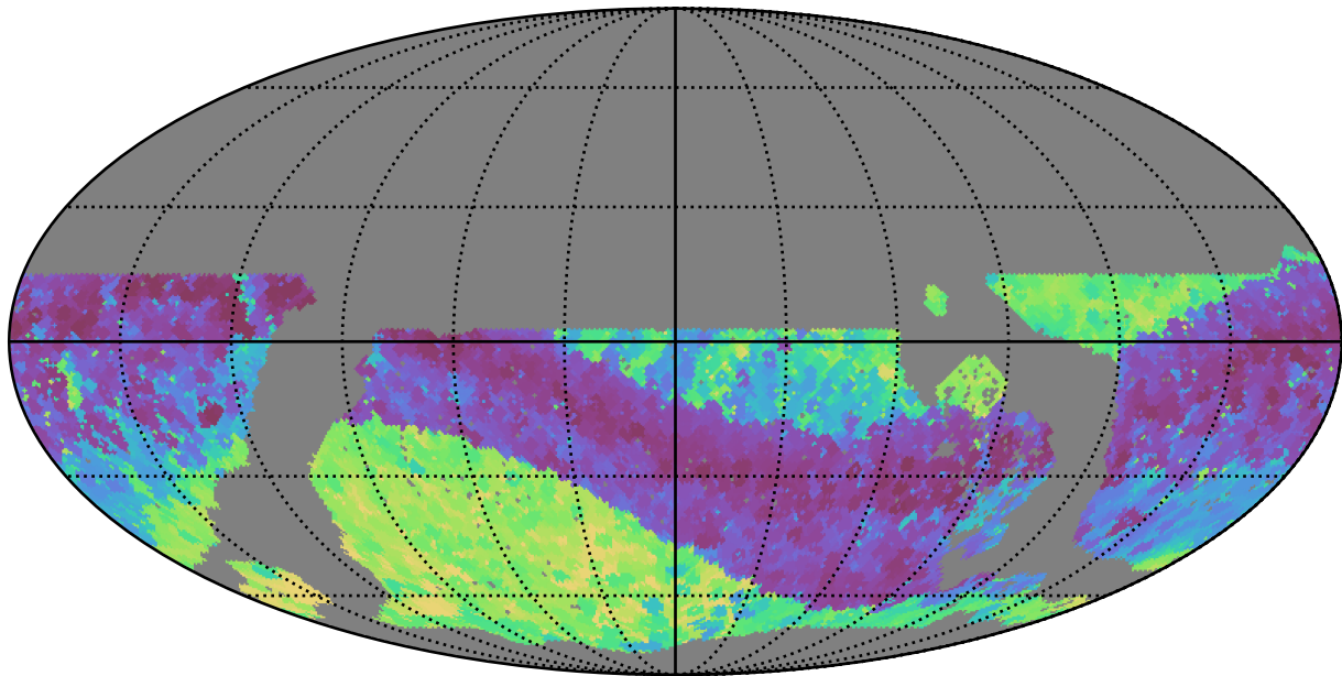
noroll_mjdp180_v3.4_10yrs WFD z band: Min skyBrightness
