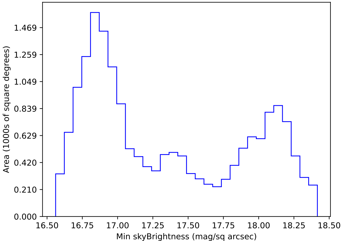
noroll_mjdp180_v3.4_10yrs WFD z band: Min skyBrightness
