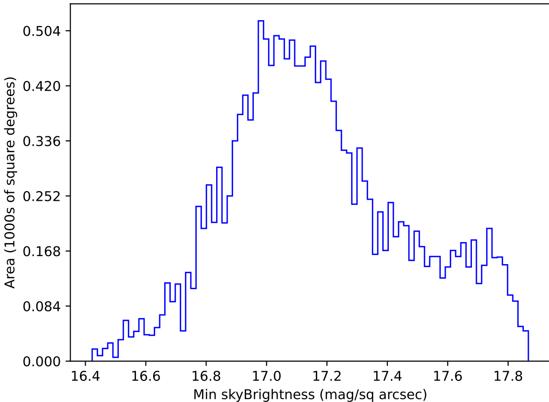
noroll_mjdp180_v3.4_10yrs WFD y band: Min skyBrightness
