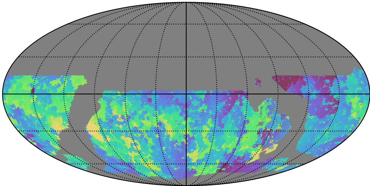
noroll_mjdp180_v3.4_10yrs WFD u band: Min skyBrightness
