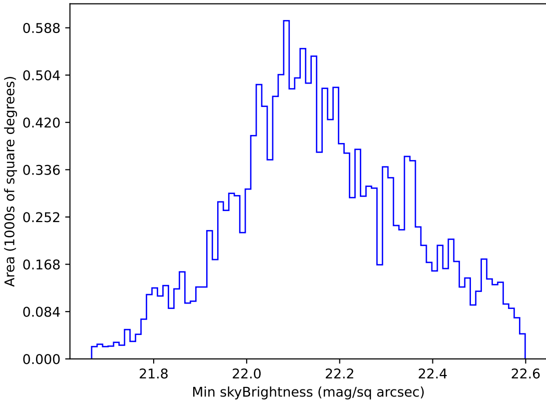
noroll_mjdp180_v3.4_10yrs WFD u band: Min skyBrightness
