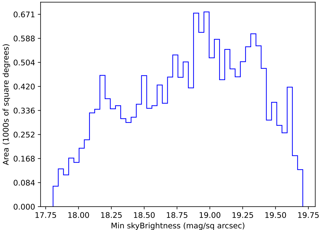
noroll_mjdp180_v3.4_10yrs WFD r band: Min skyBrightness
