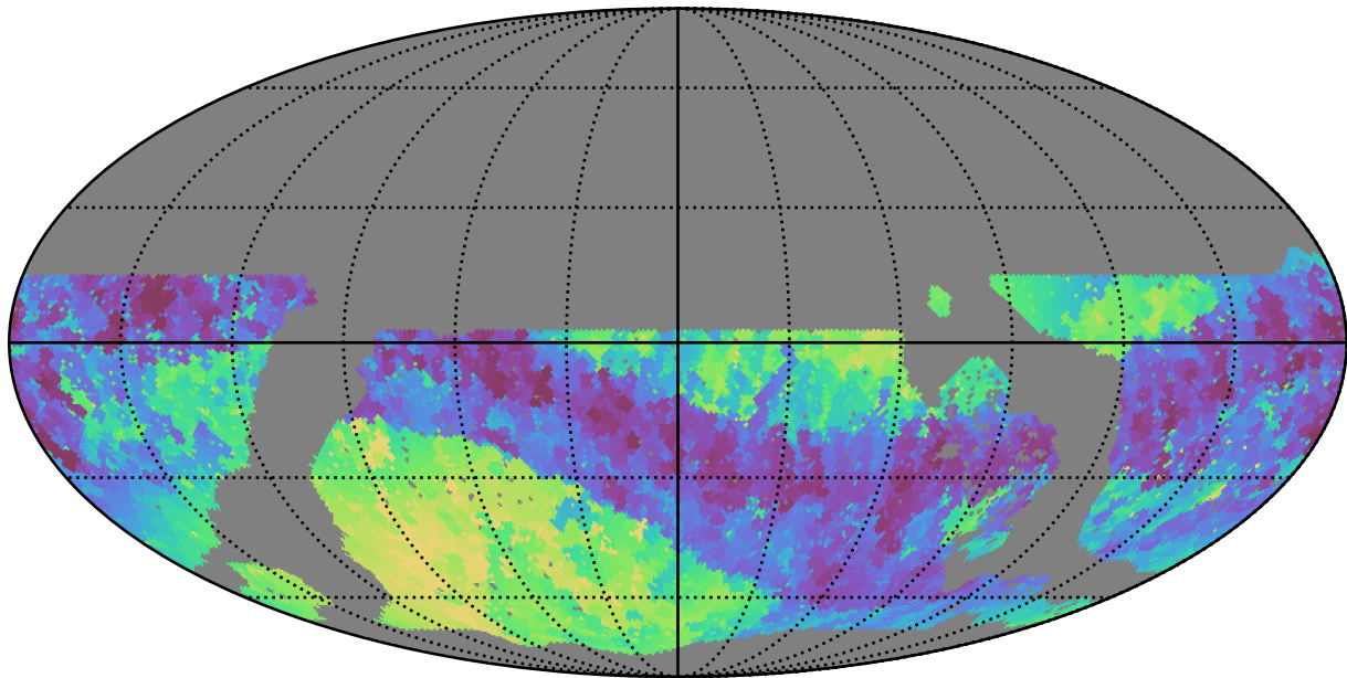
noroll_mjdp180_v3.4_10yrs WFD i band: Min skyBrightness
