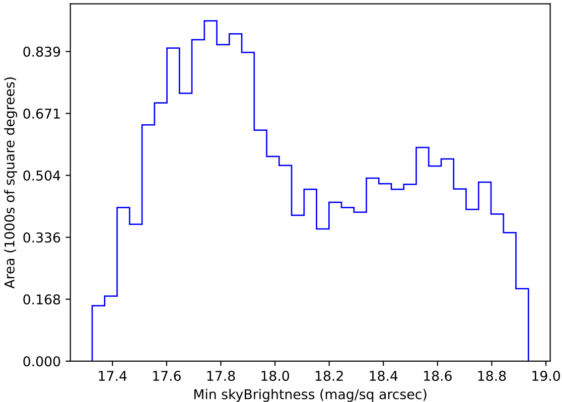
noroll_mjdp180_v3.4_10yrs WFD i band: Min skyBrightness
