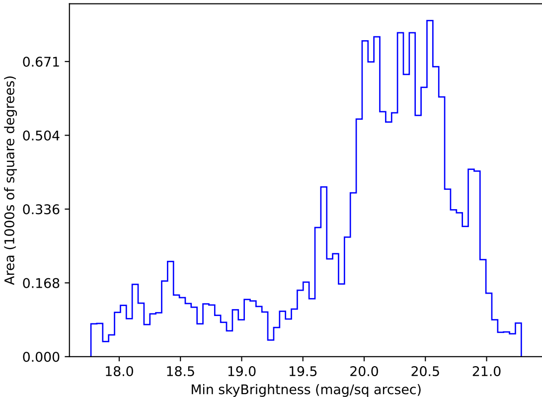
noroll_mjdp180_v3.4_10yrs WFD g band: Min skyBrightness
