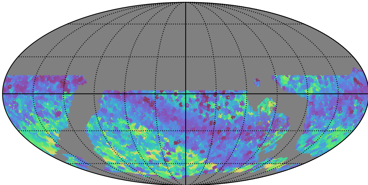
noroll_mjdp180_v3.4_10yrs WFD all bands: Min skyBrightness
