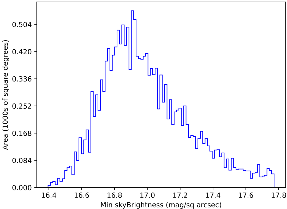
noroll_mjdp180_v3.4_10yrs WFD all bands: Min skyBrightness
