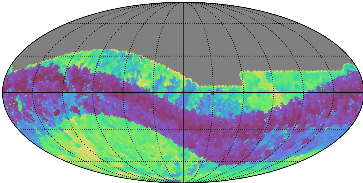
noroll_mjdp180_v3.4_10yrs All sky z band: Min skyBrightness
