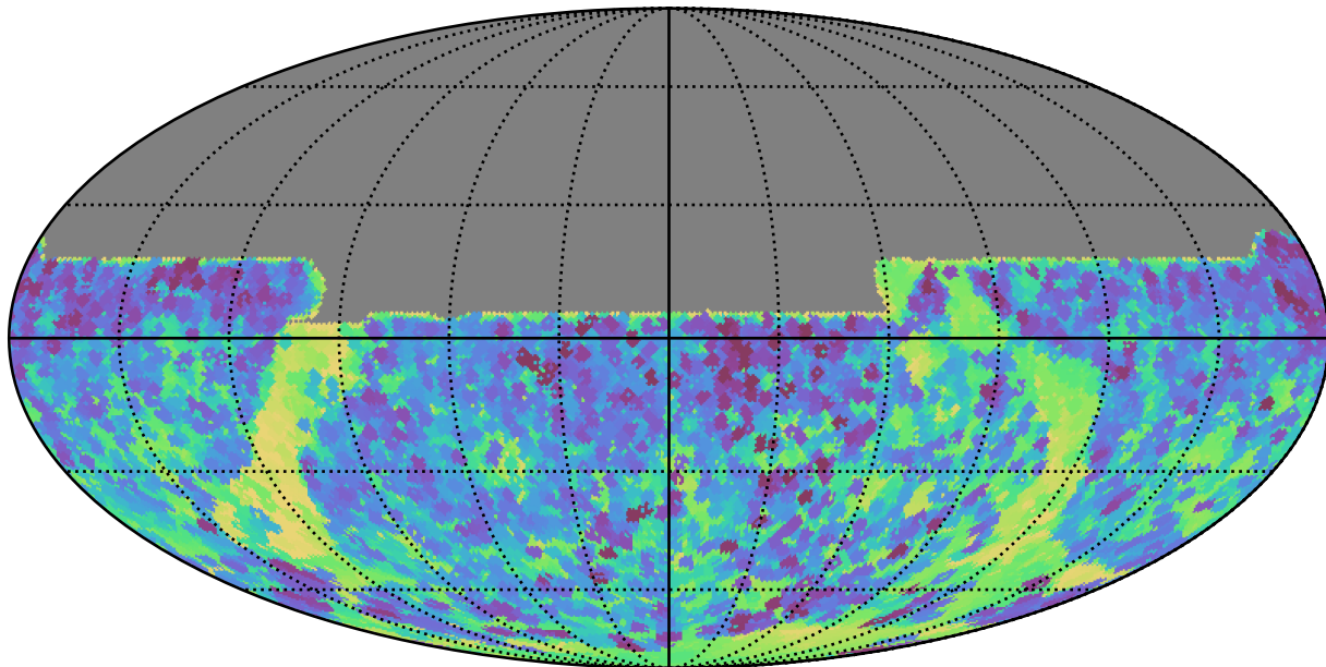
noroll_mjdp180_v3.4_10yrs All sky y band: Min skyBrightness
