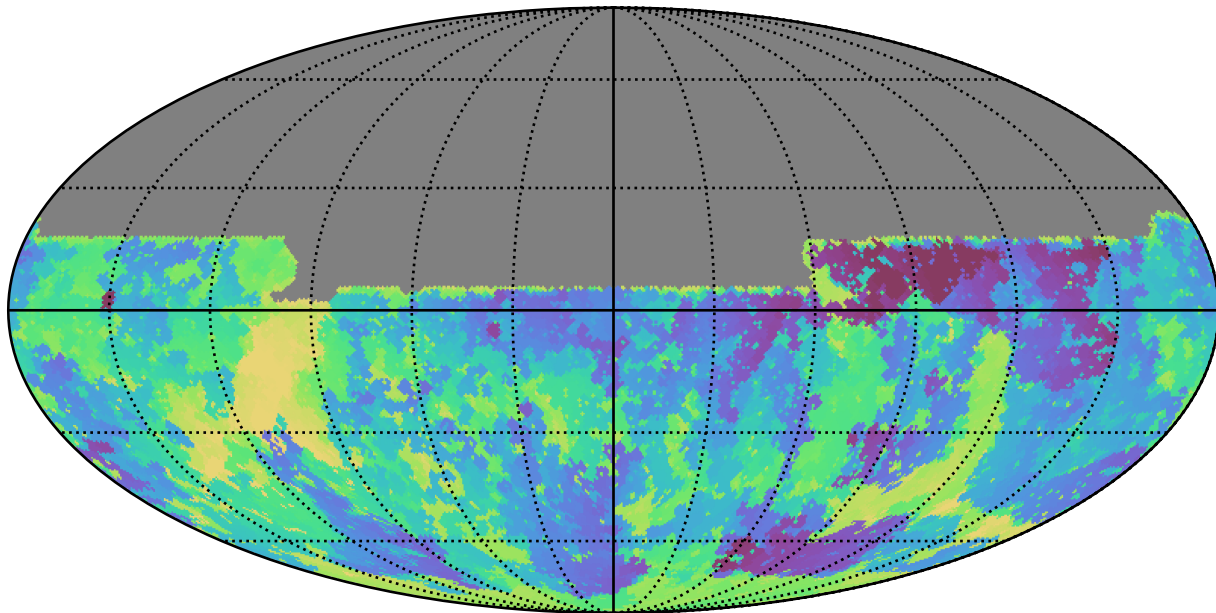
noroll_mjdp180_v3.4_10yrs All sky u band: Min skyBrightness
