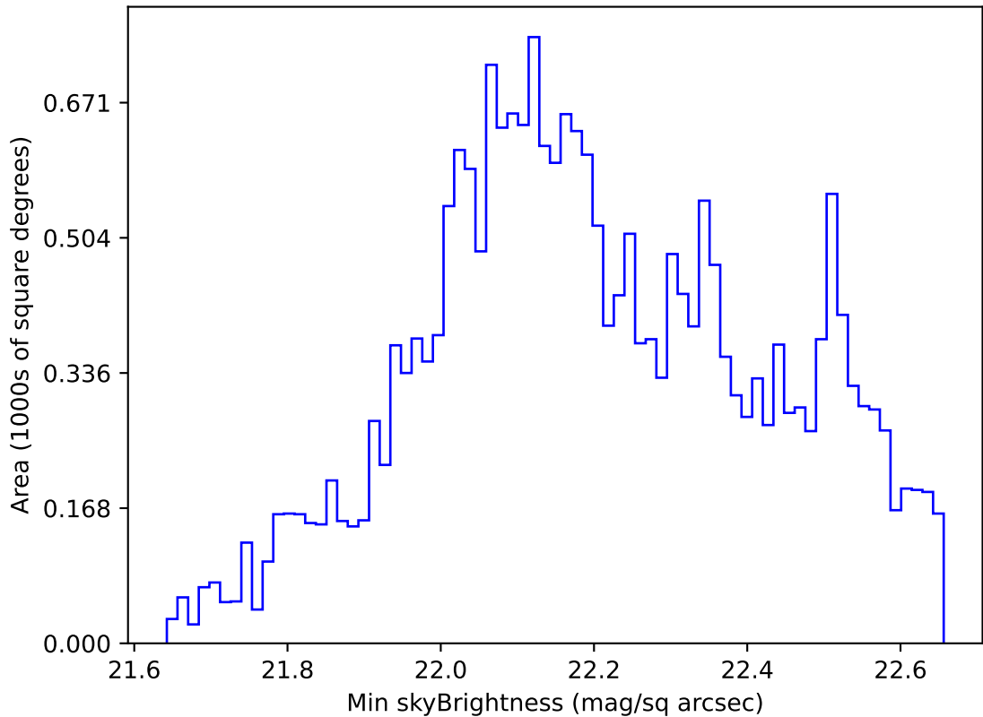
noroll_mjdp180_v3.4_10yrs All sky u band: Min skyBrightness
