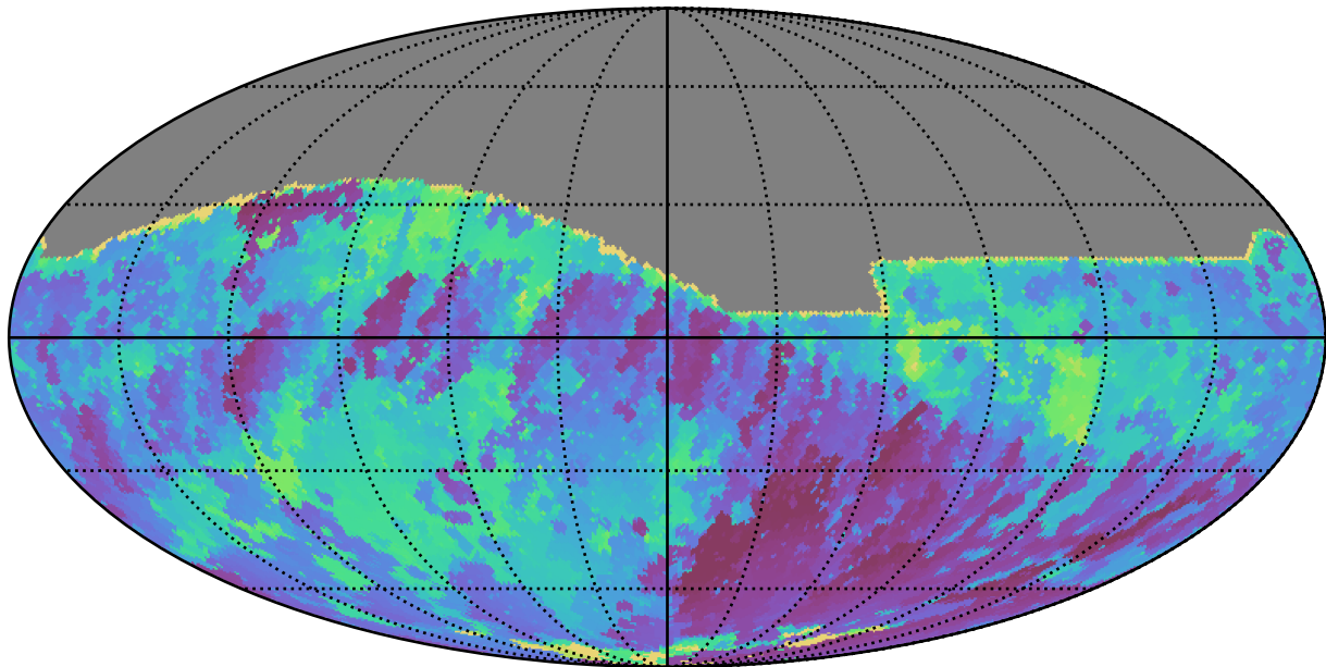
noroll_mjdp180_v3.4_10yrs All sky r band: Min skyBrightness
