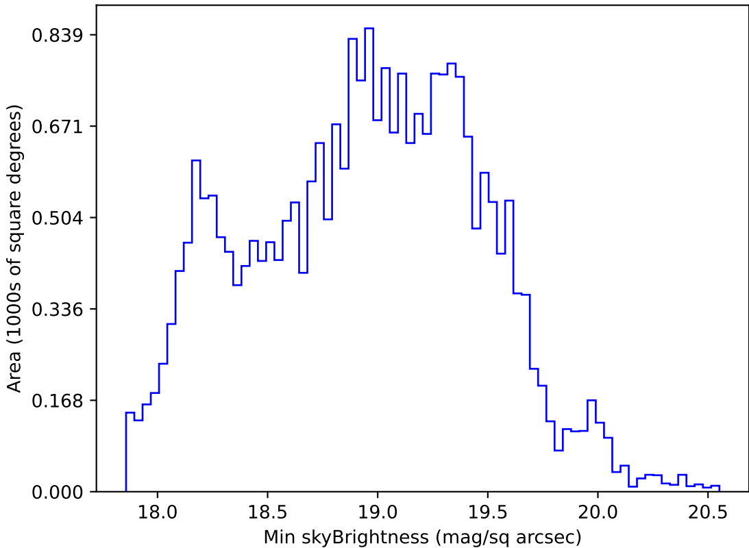
noroll_mjdp180_v3.4_10yrs All sky r band: Min skyBrightness
