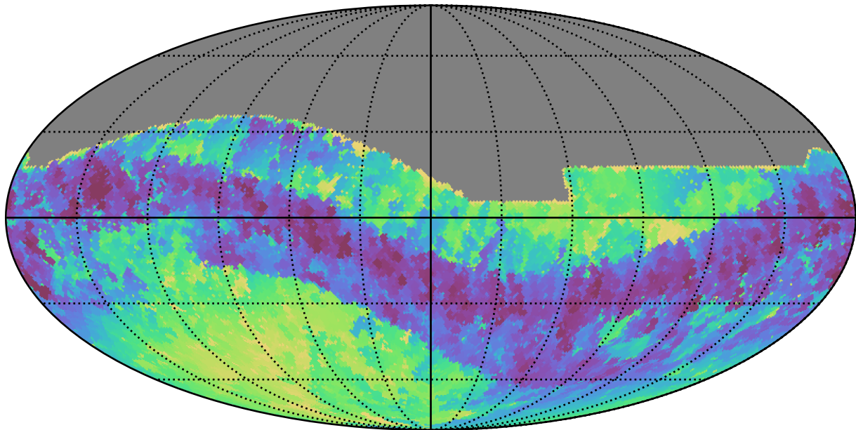
noroll_mjdp180_v3.4_10yrs All sky i band: Min skyBrightness
