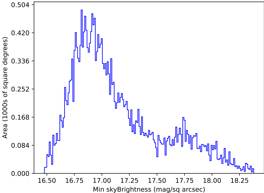
noroll_mjdp180_v3.4_10yrs All sky all bands: Min skyBrightness
