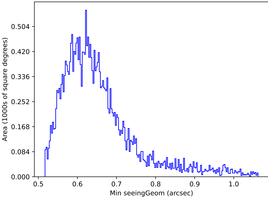
noroll_mjdp180_v3.4_10yrs Yr 1 z band: Min seeingGeom
