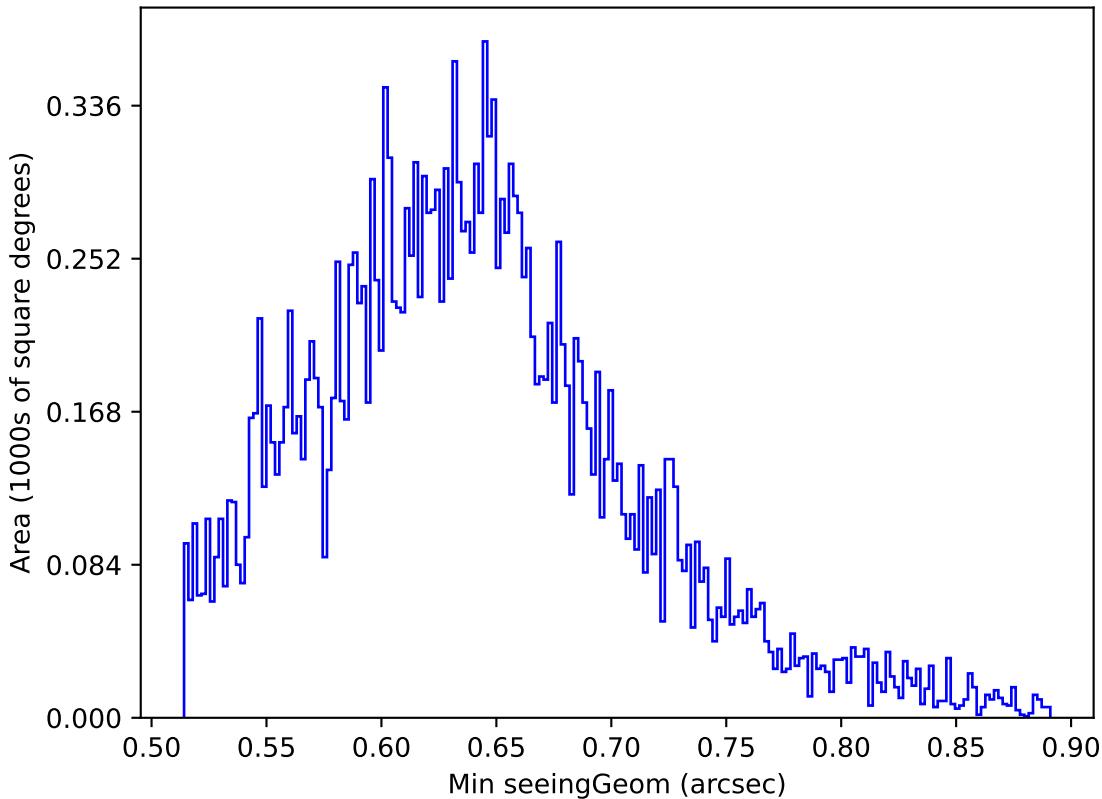
noroll_mjdp180_v3.4_10yrs Yr 1 y band: Min seeingGeom
