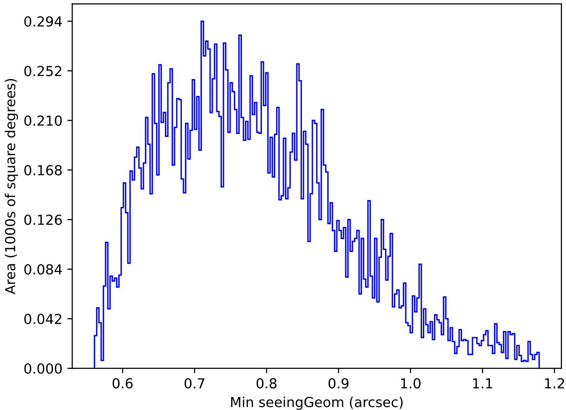
noroll_mjdp180_v3.4_10yrs Yr 1 u band: Min seeingGeom
