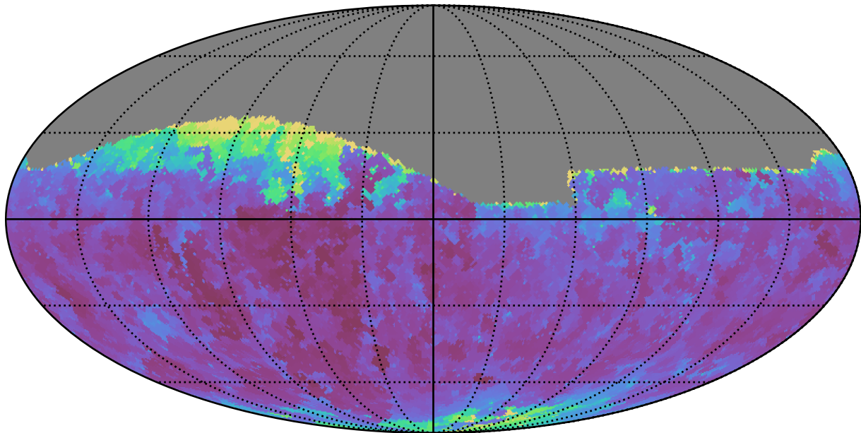
noroll_mjdp180_v3.4_10yrs Yr 1 r band: Min seeingGeom
