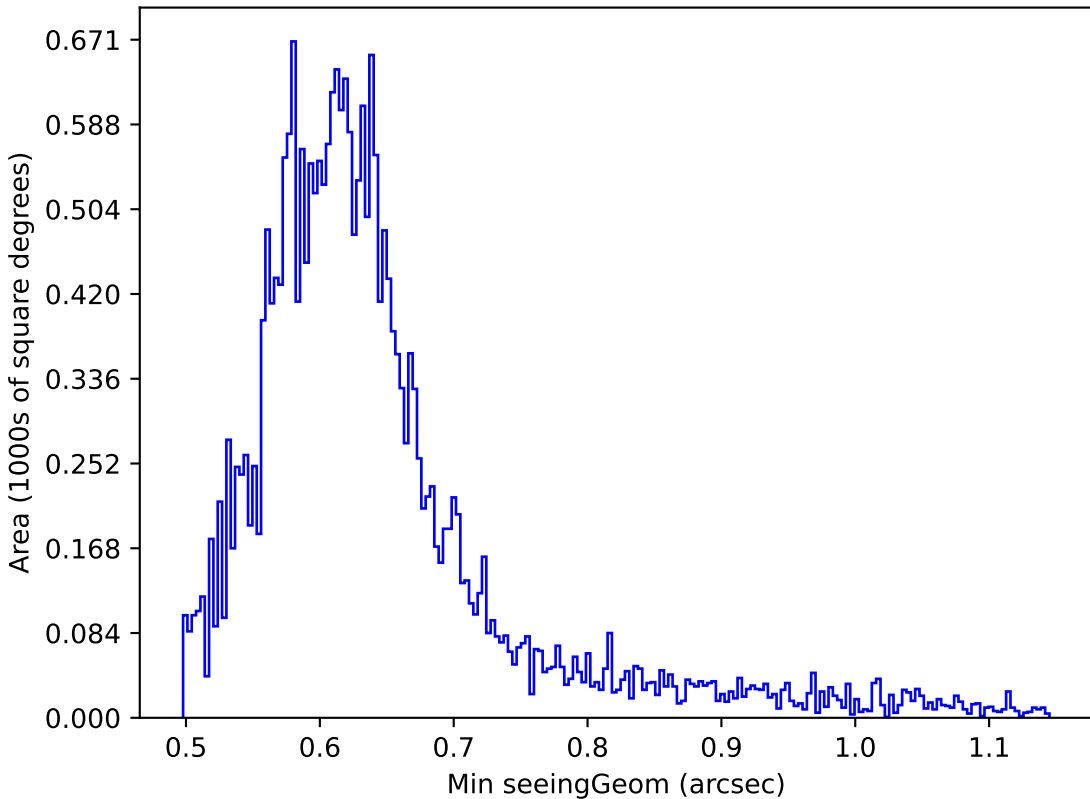
noroll_mjdp180_v3.4_10yrs Yr 1 r band: Min seeingGeom
