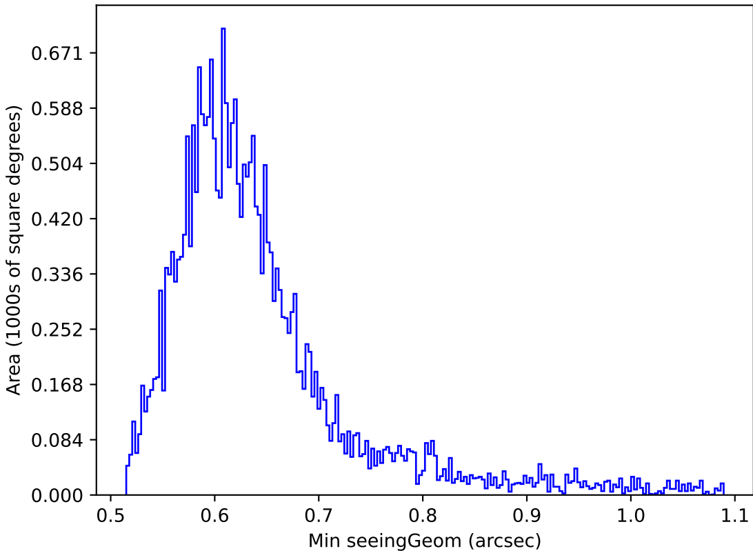
noroll_mjdp180_v3.4_10yrs Yr 1 i band: Min seeingGeom
