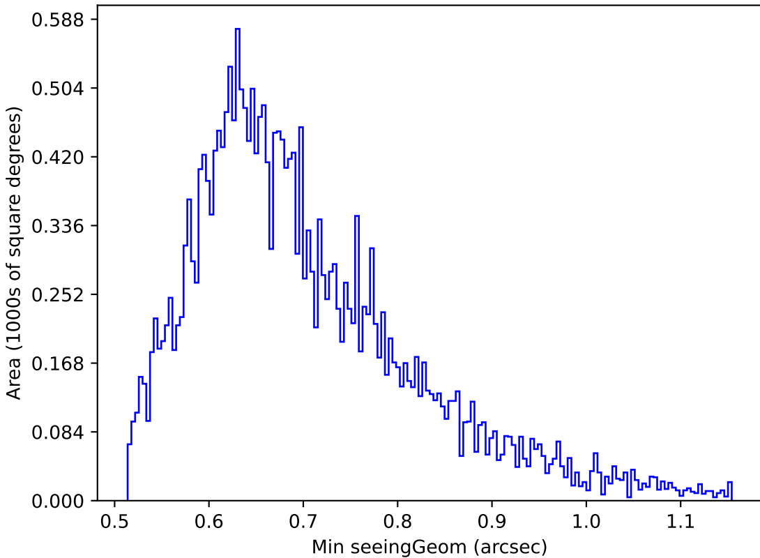
noroll_mjdp180_v3.4_10yrs Yr 1 g band: Min seeingGeom
