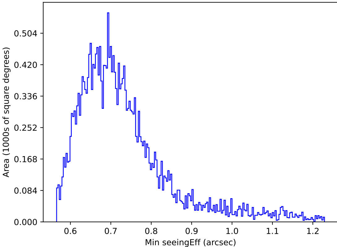
noroll_mjdp180_v3.4_10yrs Yr 1 z band: Min seeingEff
