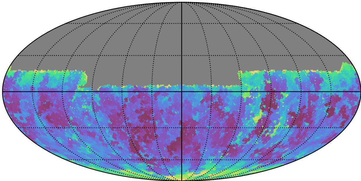
noroll_mjdp180_v3.4_10yrs Yr 1 y band: Min seeingEff
