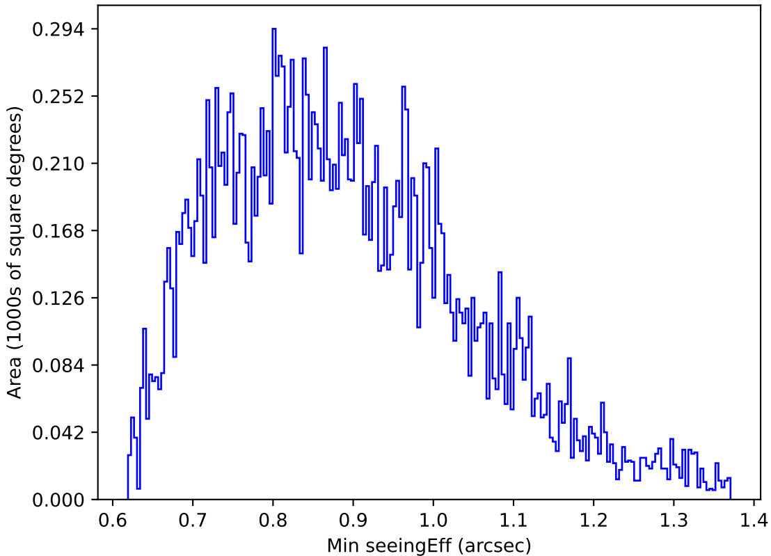
noroll_mjdp180_v3.4_10yrs Yr 1 u band: Min seeingEff
