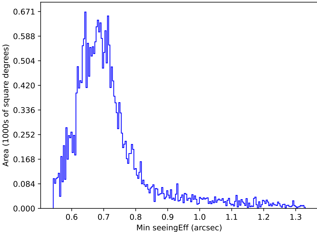
noroll_mjdp180_v3.4_10yrs Yr 1 r band: Min seeingEff
